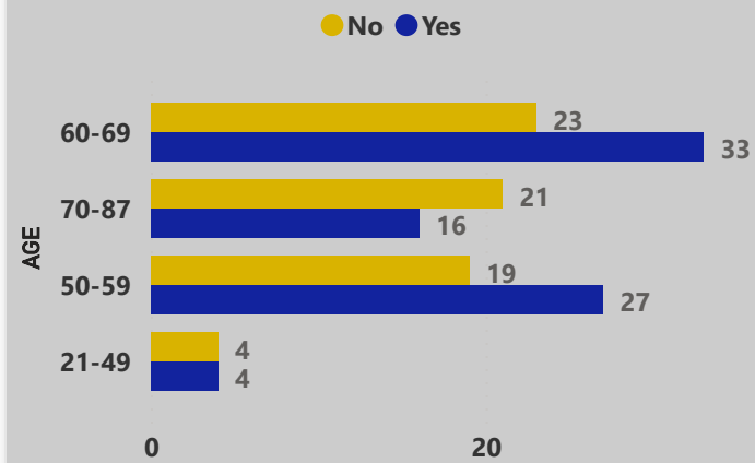
SMOKING (FEMALES)
