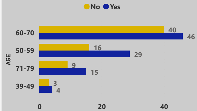
SMOKING (MALES)
